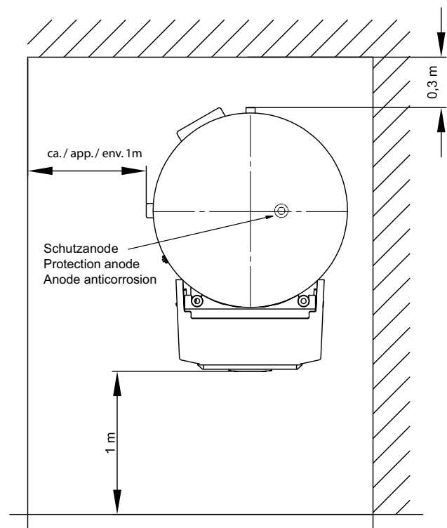
Fig. 5.1: Clearances – indoor unit
