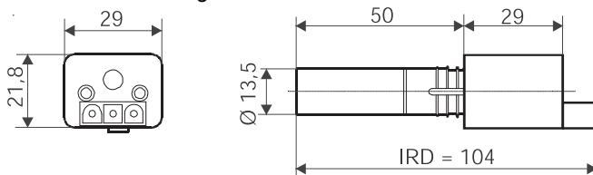
Dimensional drawing IRD 1020.1
