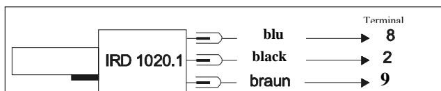
IRD 1020.1 connection
