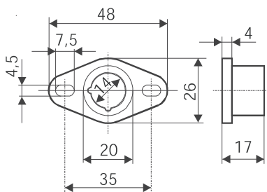
IRD 1020.1 connection
