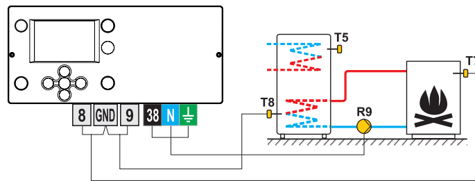
Picture 1 - D. h. w. storage tank
