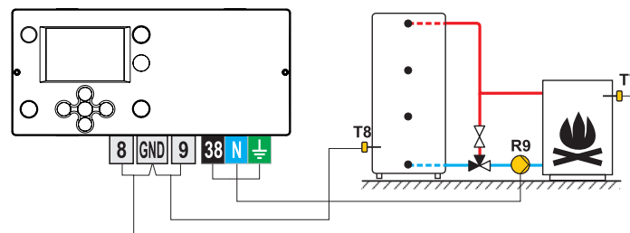
Picture 2 - Heat accumulator
