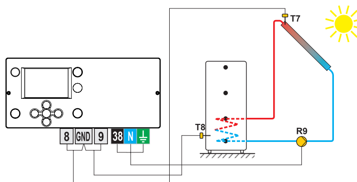
Picture 2 - Heat accumulator
