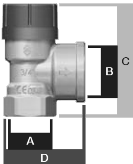
Fig. 4: Dimensions of Logafix diaphragm safety valve, ½" - 1" (dims. C, D in mm)
