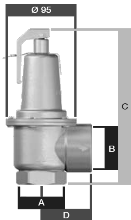
Fig. 5: Dimensions of Logafix diaphragm safety valve, 1 ¼" (dims. C, D in mm)
