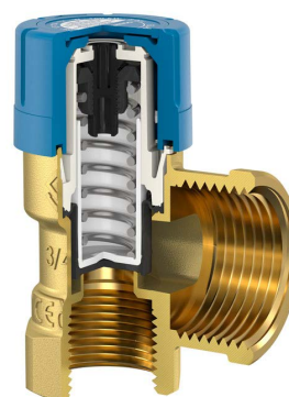
Fig. 3: Sectional model of diaphragm safety valve, 1/2" - 1"
