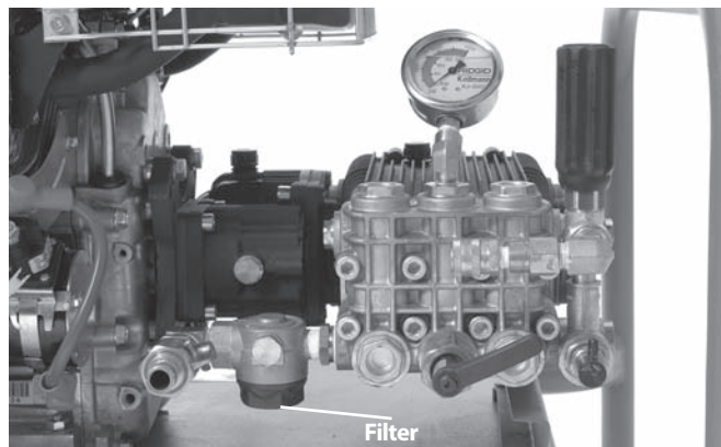
Figur 7 – Inloppsfilter/Filterbricka
