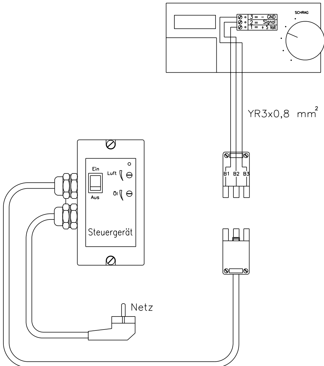
Raumthermostat RT 2001
