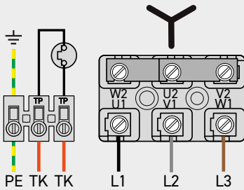
TCBT Modelle 3~ 400 V, 50 Hz, 4-315 und/4-355
