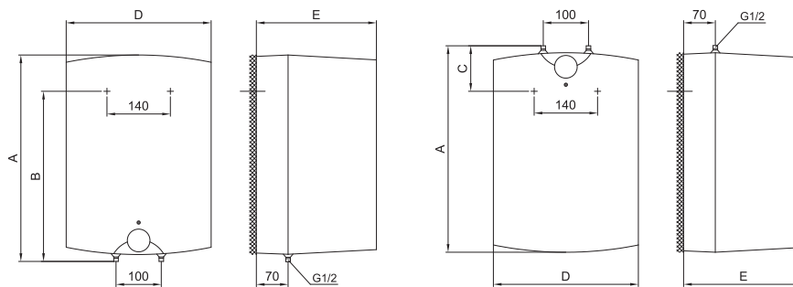
Installation above the basin/sink
