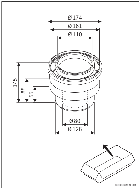
5 FC-CO110: 7738113161
