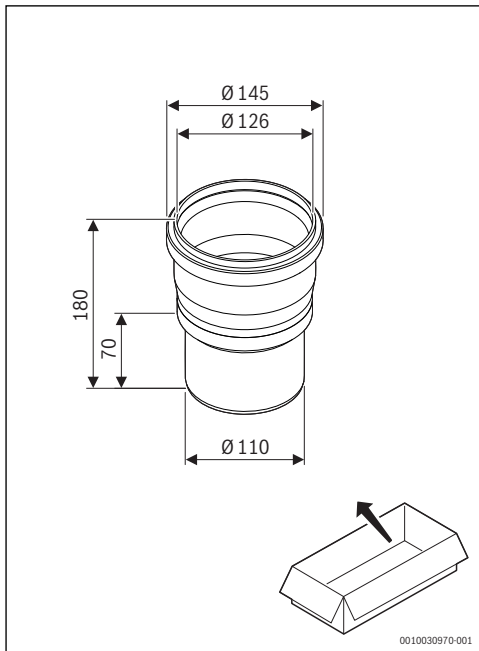
6 FC-SO125: 7738113162
