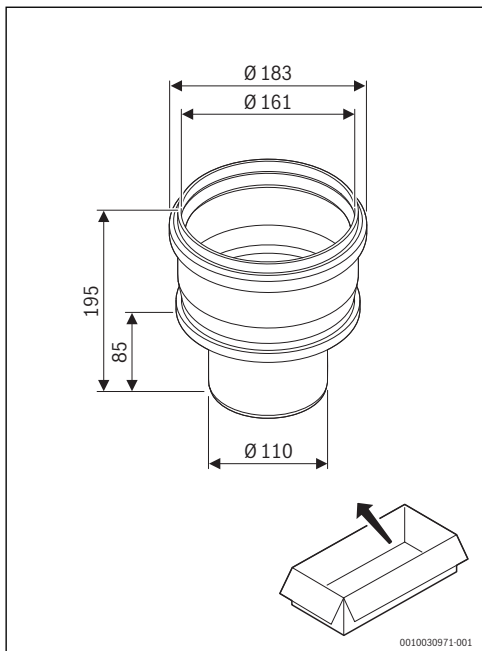
7 FC-SO160: 7738113163
